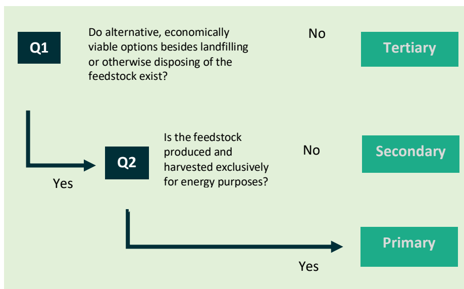
Figure 11 - Biomass Classification 19
