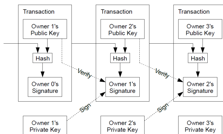
Figure 12 - Transaction flow 25
